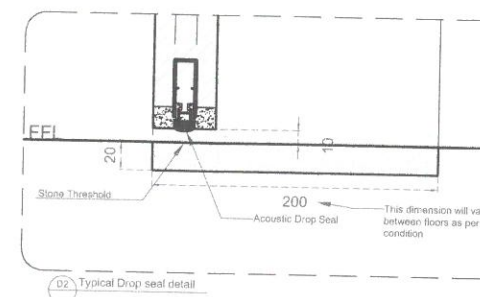
D2 Typical Drop seal detail
